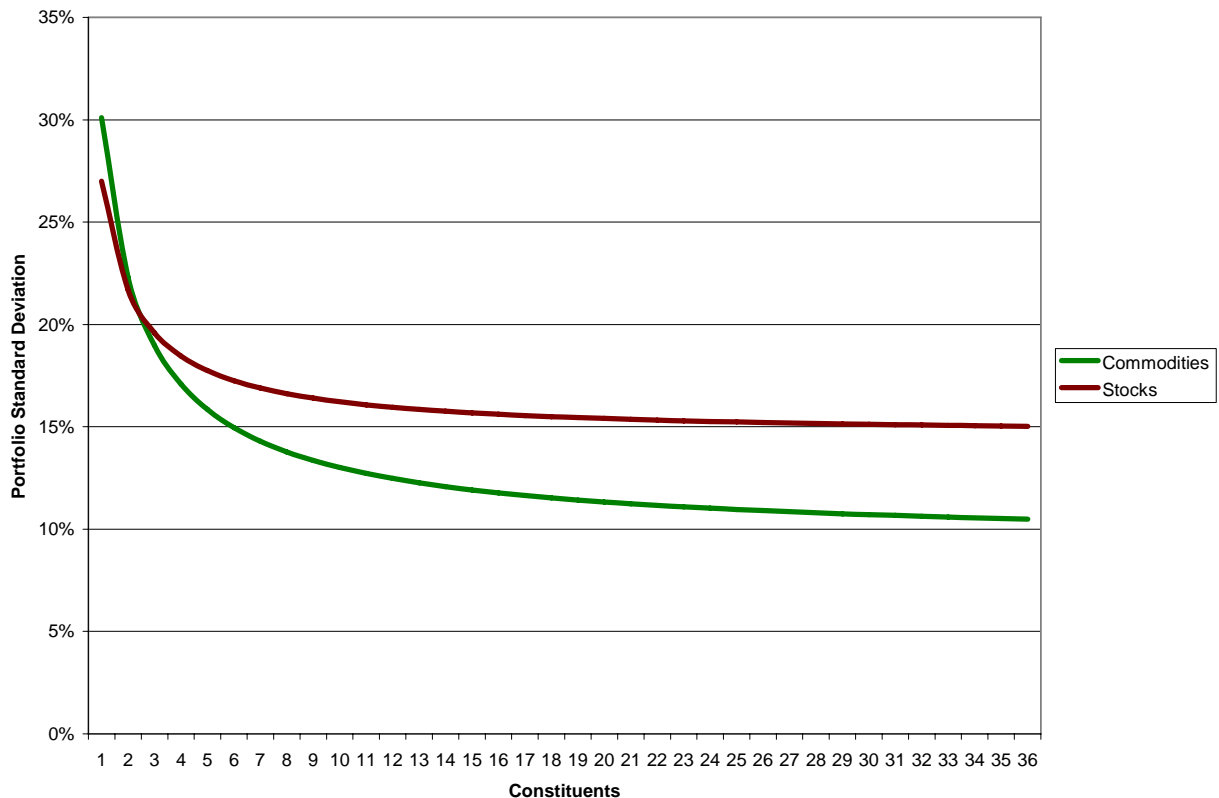
Figure 9: Evans–Archer Diversification
